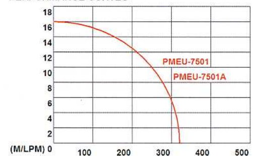
PERFORMANCE CURVES
