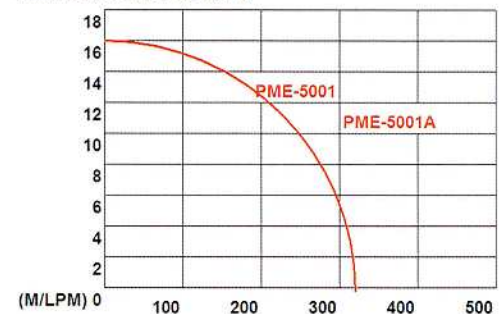
PERFORMANCE CURVES
