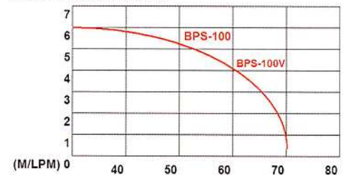
PERFORMANCE CURVES
