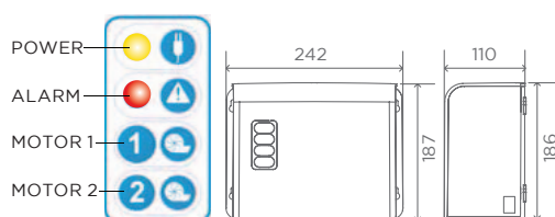
Externally mounted control box
